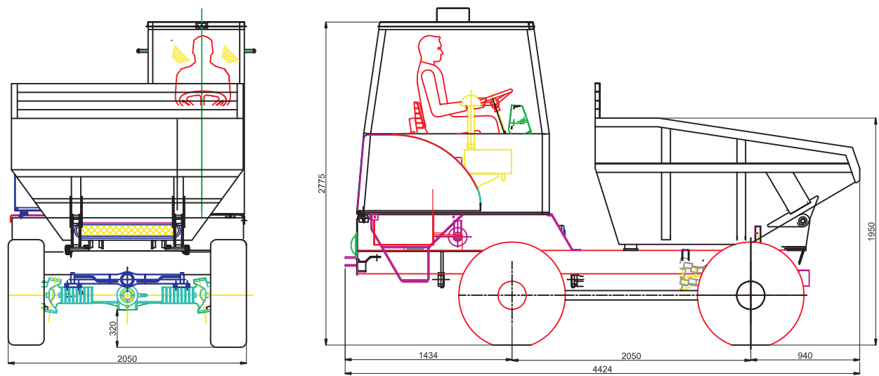
D65 6.5 ton dumper
