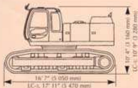
Basic machine fitted with boom and no sidewalk
