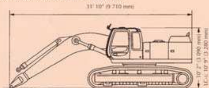
Basic machine with front and sidewalk
