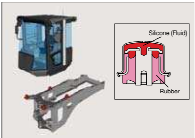
Shock-Dampened Cab
