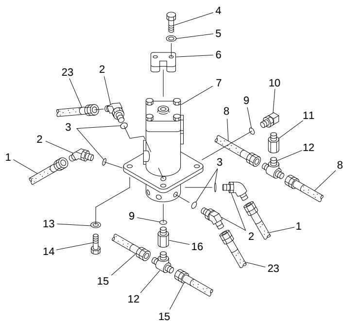
"A" DETAIL
