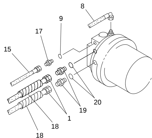
"B" DETAIL
