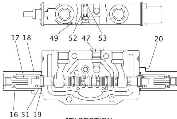
"F" SECTION
