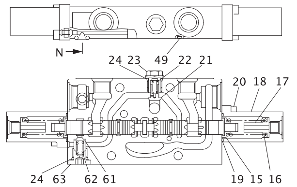
"G" SECTION
