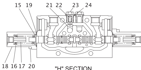
"H" SECTION
