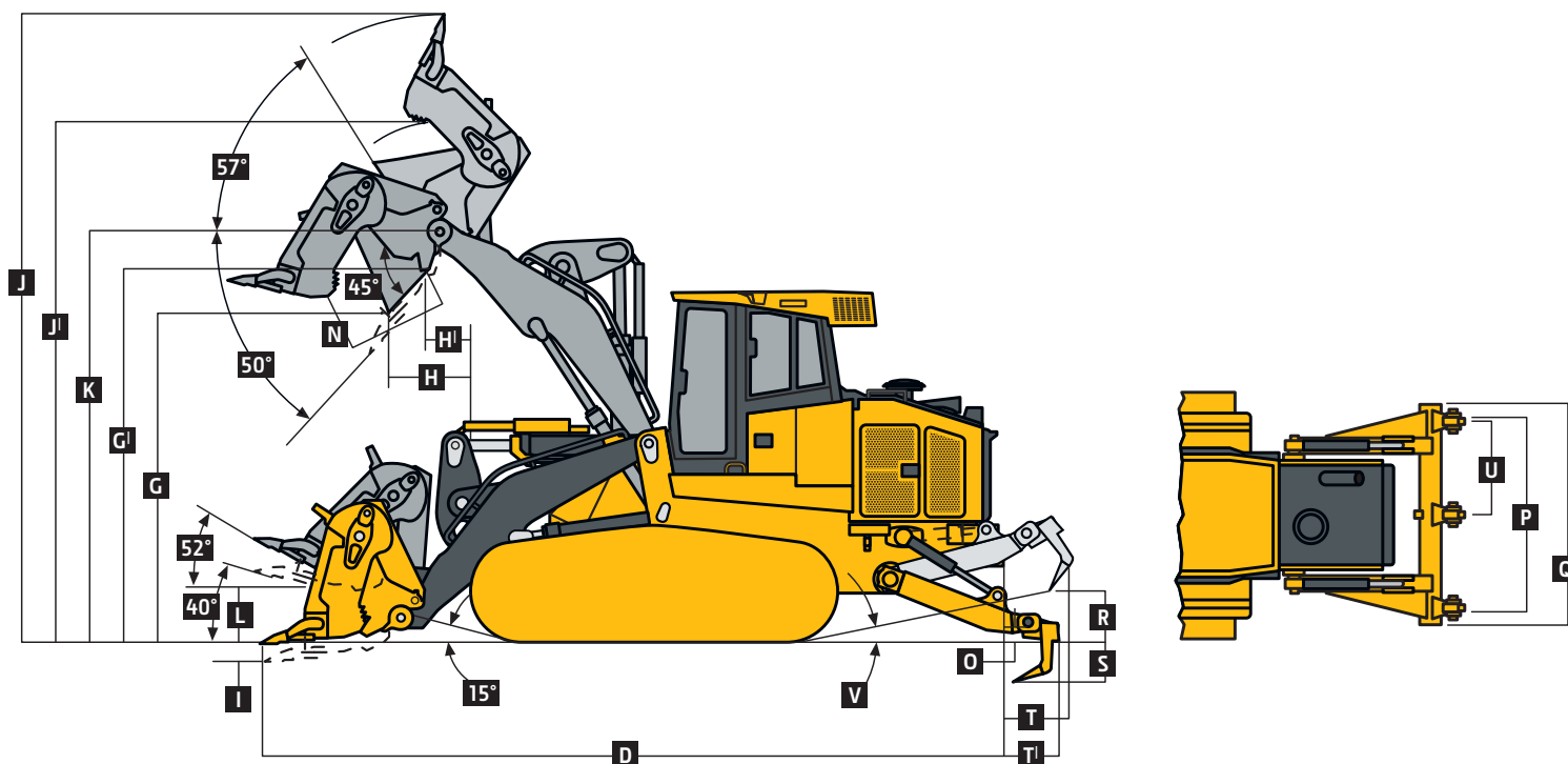
755K CRAWLER LOADER WITH MULTIPURPOSE BUCKET AND 3-SHANK RIGID-TYPE RADIAL RIPPER WITH ESCO RIPPER TIPS
