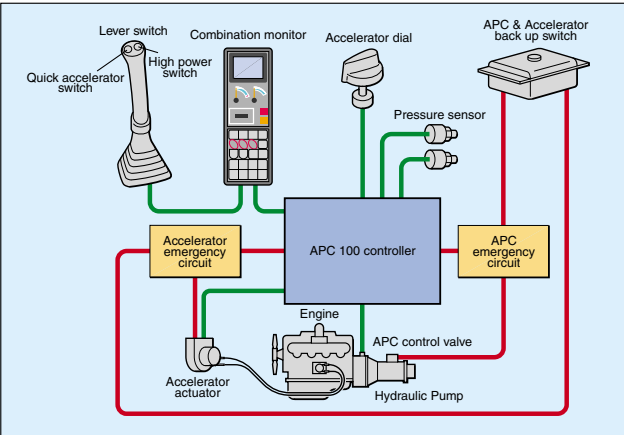
●APC(Automatic Power Control) system
